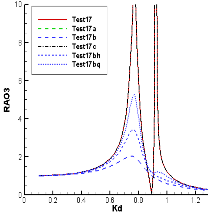
Figure A.1: Heave RAO for each of the test17 runs. The results for Test17, Test17a, and Test17c are practically identical. The results for Test17b (lid with damping) include three values of the external damping coefficients. In Test17b b_{33} = 0.4 and b_{77} = 0.1 , as shown in the test17b.frc file below. In Test17bh these values are reduced by a factor of one-half and in Test17bq they are reduced by a factor of one-quarter.
