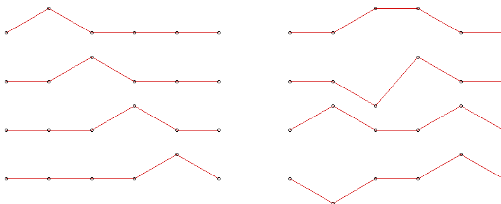
Figure A.3: Generalized modes used for the hinged barge with four hinges. The modes on the left are ‘tent functions’, suitable for use when ISX=0. When ISX=1 each mode must be either symmetric or antisymmetric, as shown in the right column. The latter modes are used for TEST24. The conventional rigid-body modes in heave and pitch represent the nonzero vertical motions at the two ends.
