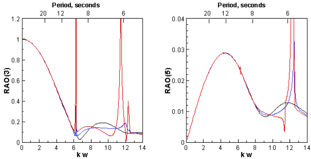
Figure A.2: Heave and pitch RAO's of the MultiSurf Barge as computed in TEST20a . The black lines are the RAO's in a fluid domain of infinite width. The red lines are the RAO's in a channel of width w = 100\text{m} and depth 15\text{m} . Resonant standing waves occur near kw = 2\pi and kw = 4\pi , where k = 2\pi/\lambda is the finite-depth wavenumber and \lambda is the wavelength. The blue lines show the results when the parameter CHANNEL_REFLECT = 0.5 is used, to reduce the effect of the wall reflections near resonance.
